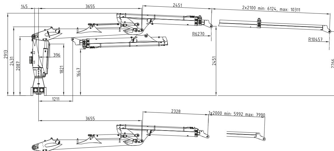
170° Hochklappung 170° of lifting up
