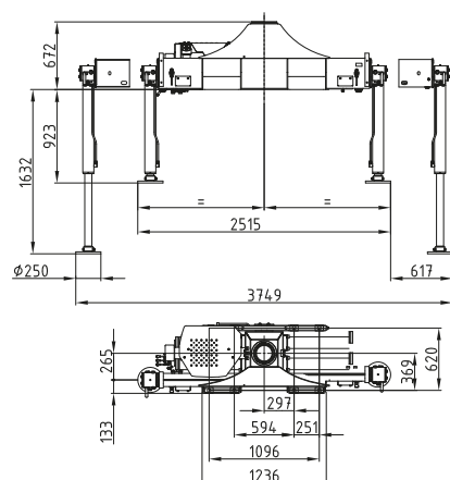
Kransockel schmal Crane base small
