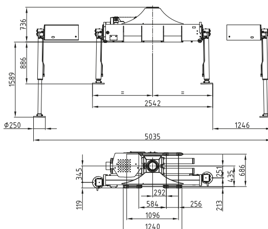
Kransockel breit Crane base wide
