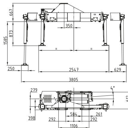
Kransockel Standard Crane base standard
