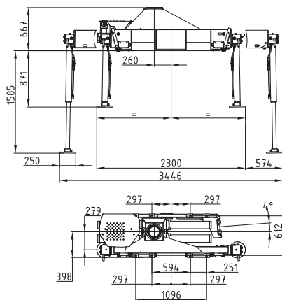
Kransockel Schmal Crane base narrow
