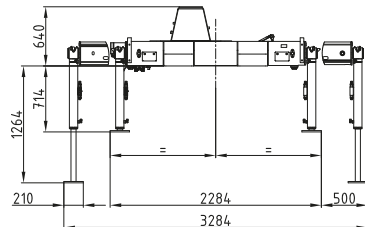
Kransockel Standard Crane base standard
