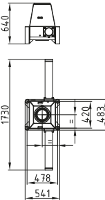
Kransockel mittig Crane base centered
