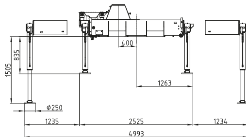
Socket Crane base
