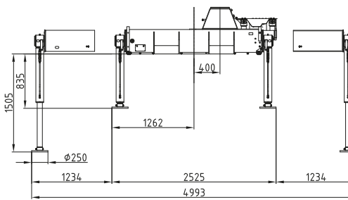
Socket side inverted Crane base inverted
