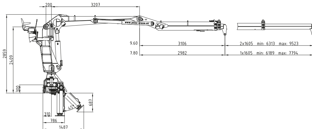
Sockel Crane base
