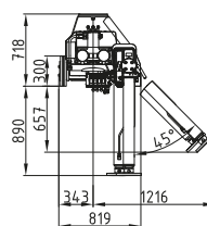
Kransockel 5000mm Crane base 5000mm
