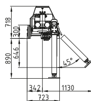
Kransockel 3800mm Crane base 3800mm
