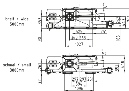
Kransockel 5000mm Crane base 5000mm
