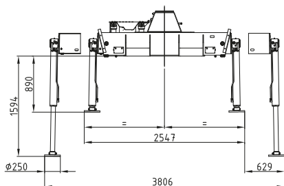
Sockel schmal Crane base small
