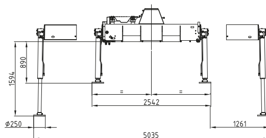
Sockel breit Crane base wide
