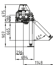
Kransockel 3800mm Crane base 3800mm
