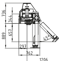
Kransockel 5000mm Crane base 5000mm
