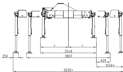
Kransockel Crane base
