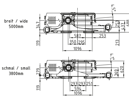
Kransockel 3800mm Crane base 3800mm
