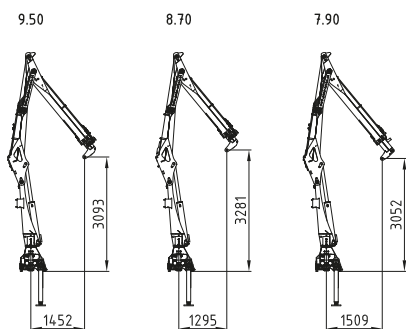
Kransockel Crane base
