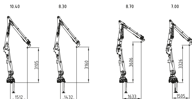
Kransockel *Kransockel 5000mm Crane base 5000mm
