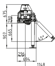
Kransockel 3800mm Crane base 3800mm
