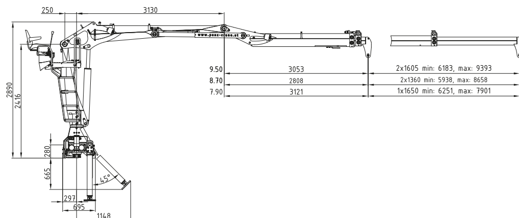
Kransockel •Kransockel 5000mm Crane base •Crane base 5000mm
