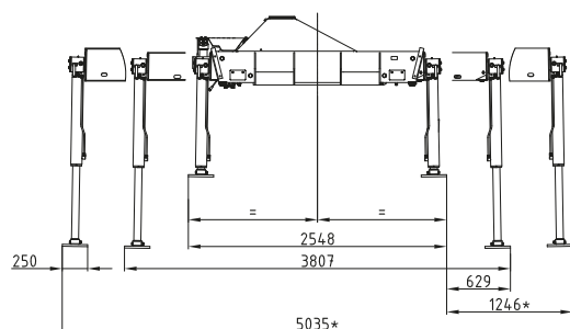
Kransockel •Kransockel 5000mm Crane base •Crane base 5000mm
