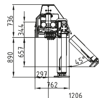
Kransockel 5000mm Crane base 5000mm
